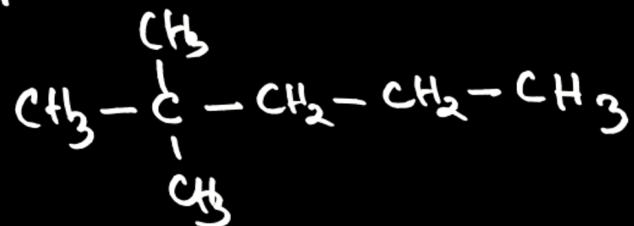
neo-heptane
